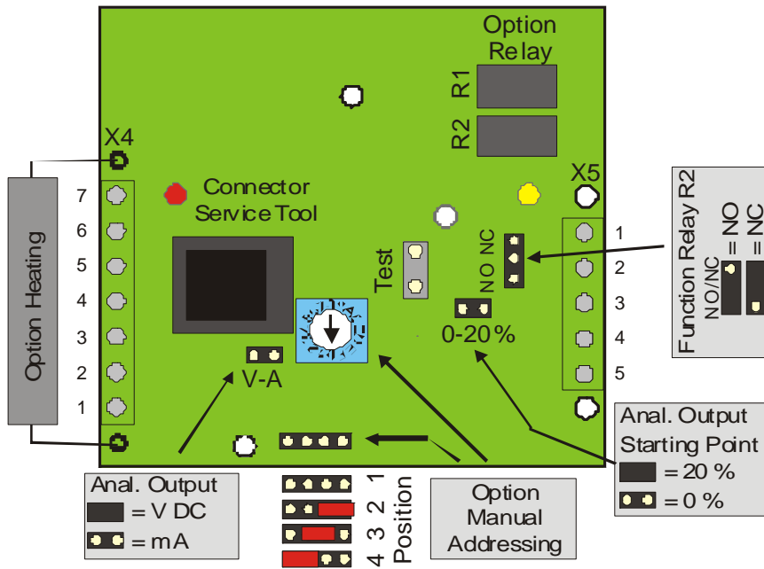
PCB SM03
